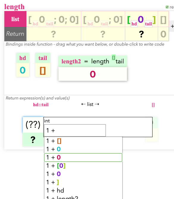
■ Figure 8 Autocompleting to a value in scope.
