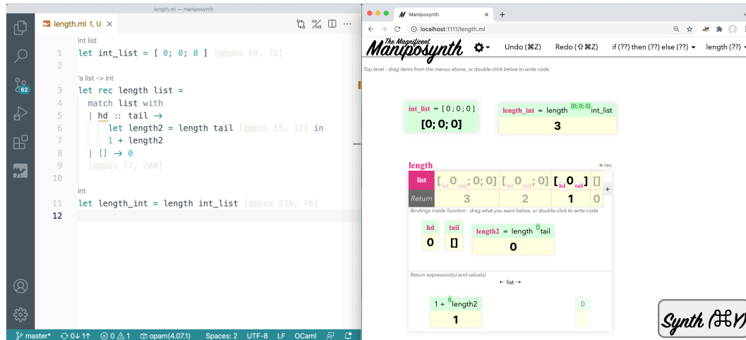
Figure 1 A list length function implemented in MANIPOSYNTH.
