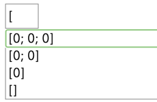
■ Figure 2 List literals in autocomplete menu.
